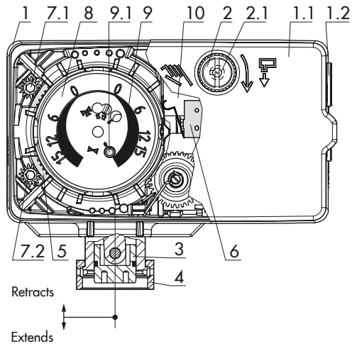
Fig. 2: Design of Type 5827 (force-locking attachment)
