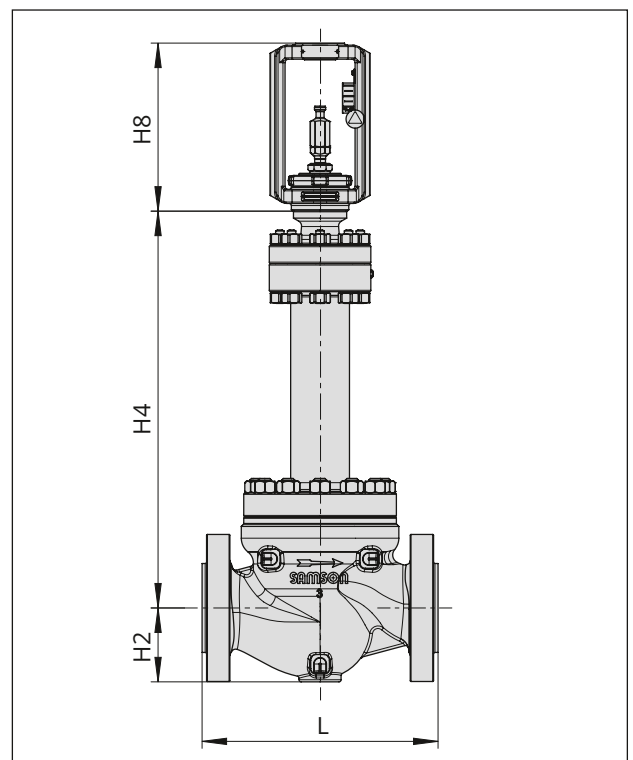
Fig. 8: Type 251GR Valve with bellows seal
