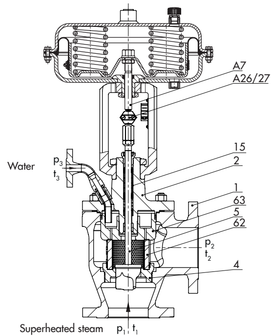
Fig. 3: Type 3286 Steam Conditioning Valve with Type 3271 Pneumatic Actuator
