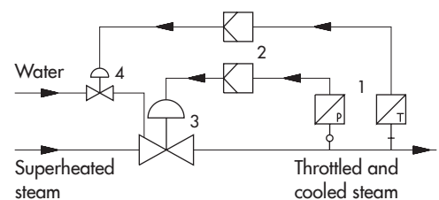
Fig. 1: Type 3286-1 Pneumatic Steam Conditioning Valve
